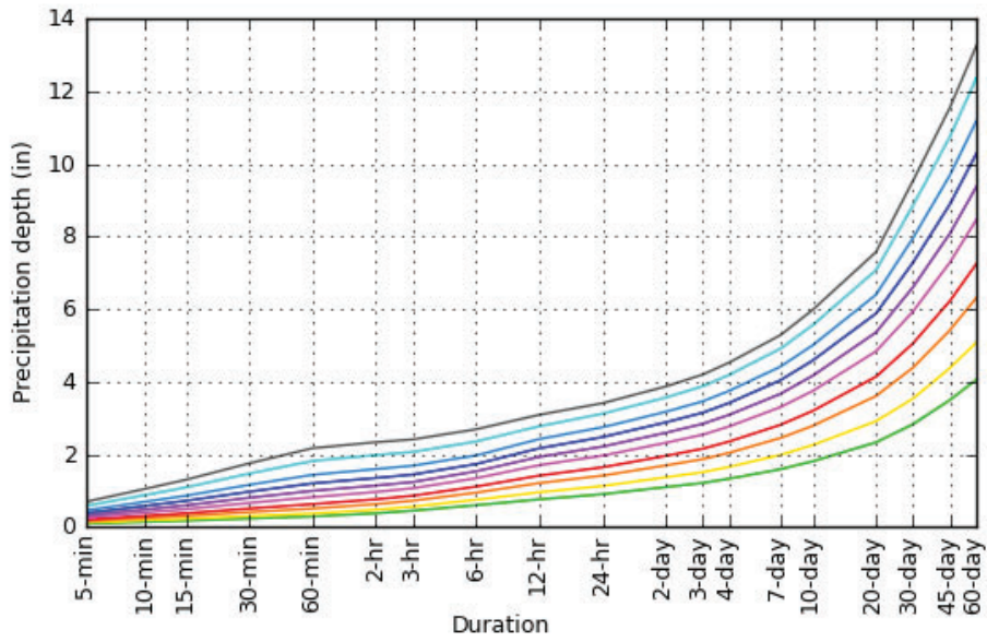
PDS-based depth-duration-frequency (DDF) curves Latitude: 41.6960°, Longitude: -118.0206°
